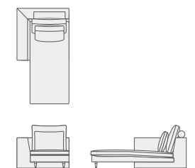
One arm couch W980 D1800 H850 SH400
