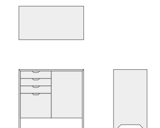
1 door & 4 drawers W870 D450 H800
