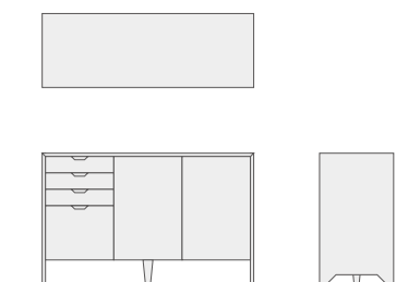
2 doors & 4 drawers W1285 D450 H800
