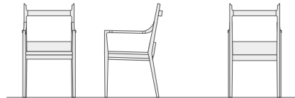
arm W500 D540 H880 SH440 AH630
