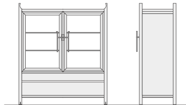
2 glass doors & 2 drawers W1200 D500 H1380
