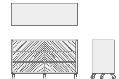
Front & Back sides use W1800 D600 H1075
