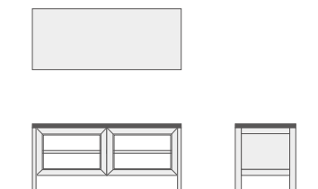
2 glass doors W1100 D500 H500
